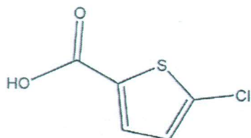
5-Chloro-2-thiophene carboxylic acid
