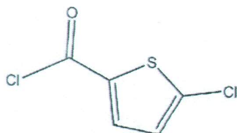
5-Chlorothiophene-2-carbonyl chloride
