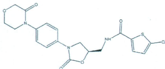
5-Chloro-N-[[[(5R)-2-oxo-3-[4-(3-oxo-4-morpholinyl)phenyl]-5-oxazolidinyl] methyl]-2-thiophene carboxamide
